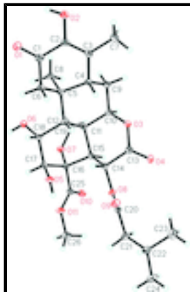
Fig. 1. Ellipsoid plot.
